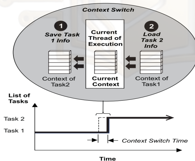
Figure 5-3: Multitasking using a context Switch
